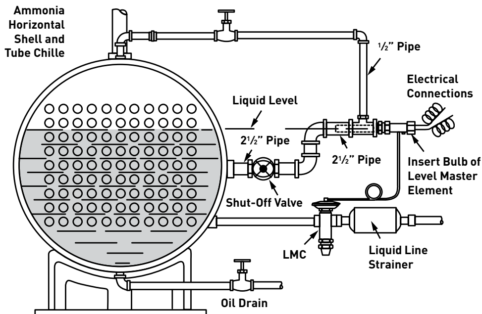
Figure 4: Typical Installation
