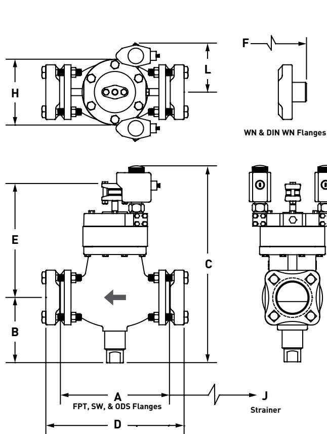
Dimensional Diagram: CK-2D Dual Position Gas Powered Suction Stop Valves
