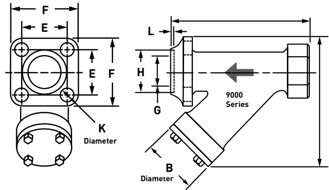
Dimensional Diagram: 9000 Series Strainer
