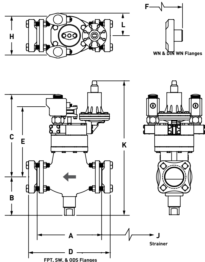
Dimensional Diagram: CK-6D Dual Position Gas Powered Suction Stop Valves
