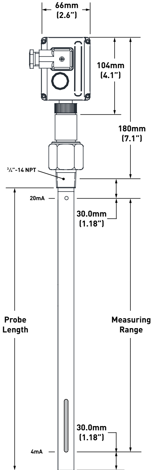
Dimensional Diagram: Liquid Level Transmitter (HBLT-A1)
