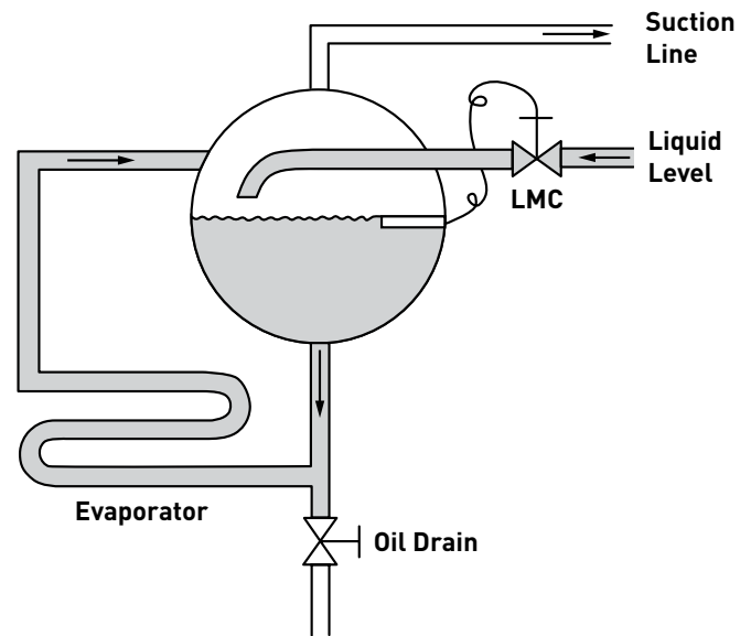
Figure 3: Surge Drum
